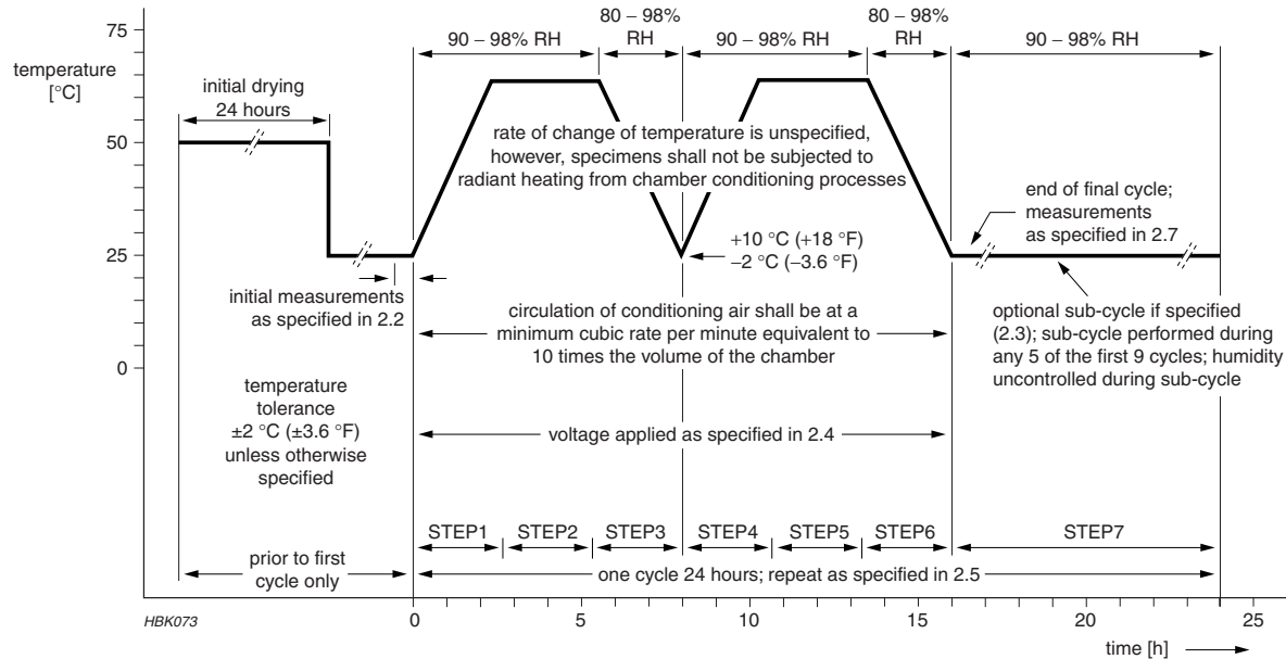
Fig. 8 Moisture resistance test requirements
